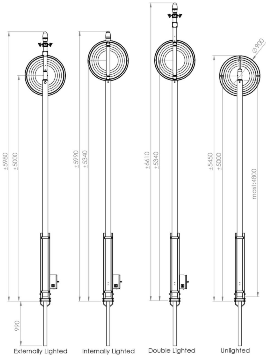
STYLE I-B: INTERNALLY LIGHTED
